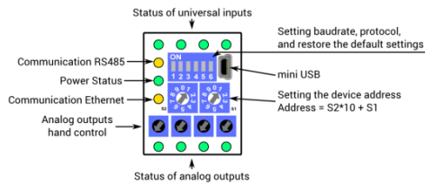
Figure 13. Top panels 4U4A-H and 4U4A-H-IP
