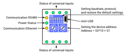
Figure 10. Top panels 8U and 8U-IP
