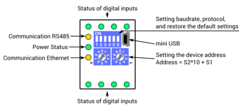
Figure 9. Top panels 8I and 8I-IP
