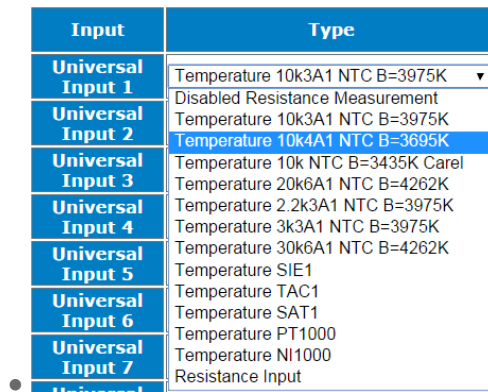
Figure 34. Types of sensors
