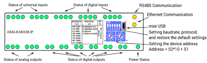
Figure 8. Top panel MIX38-IP
