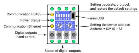
Figure 14. Top panels 40-H and 40-H-IP
