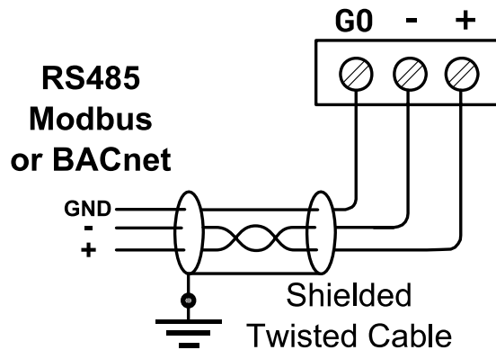
Figure 6. RS485 connection
