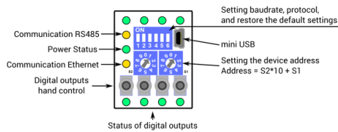
Figure 15. Top panels 4TO-H and 4TO-H-IP
