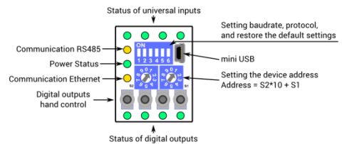
Figure 12. Top panels 4U40-H and 4U40-H-IP
