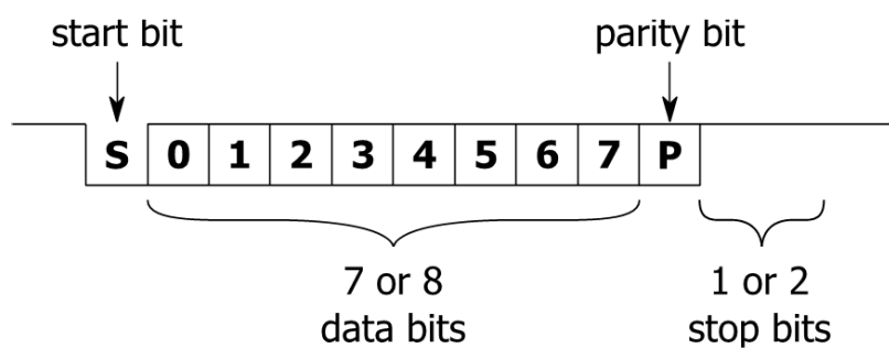
Figure 12 Modbus message frame
