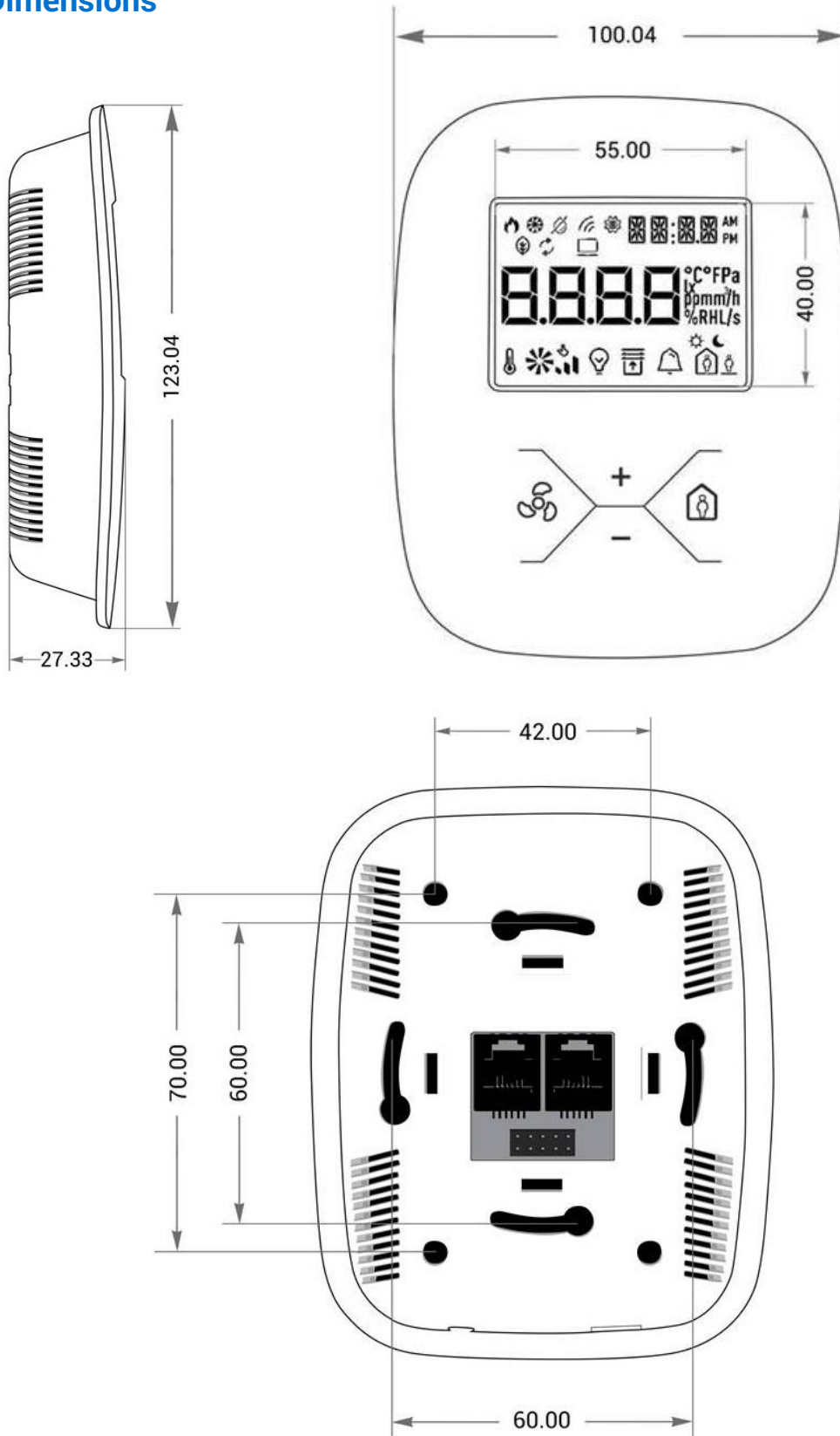
Figure 1 Room Panel iSMA-B-LP dimensions
