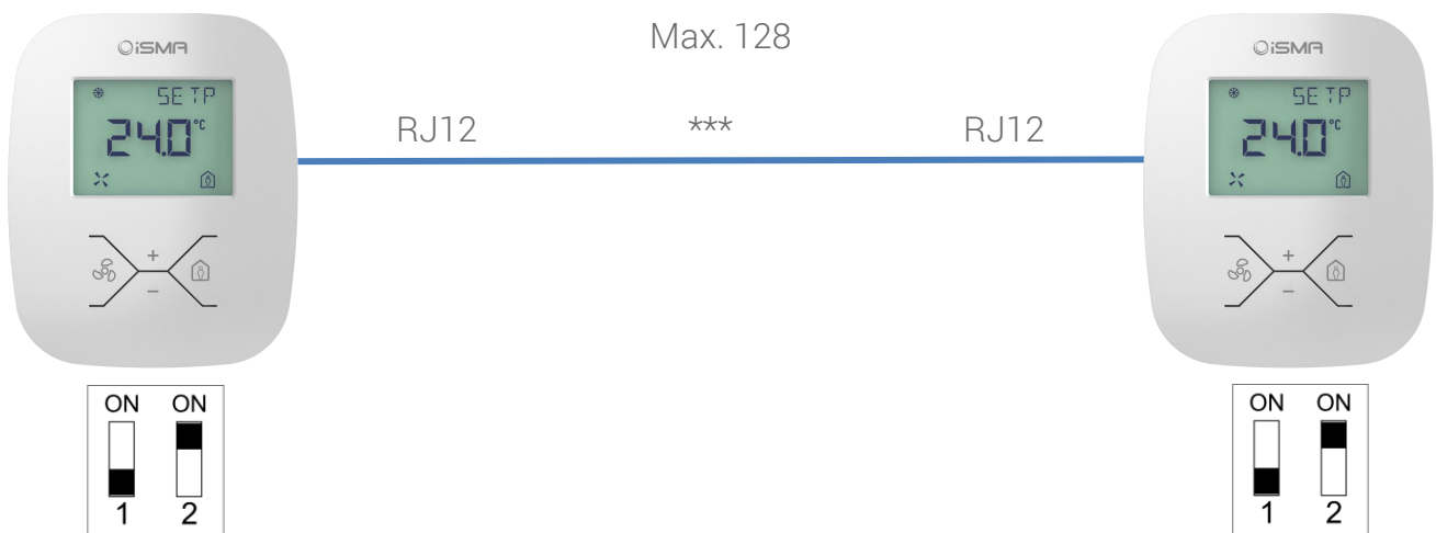
Figure 7 Several Room Panels connection
