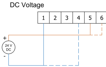
Figure 4 DC power supply connection
