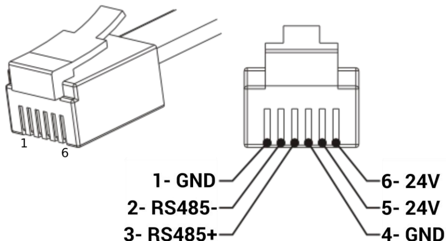
Figure 3 RJ12 socket pin configuration
